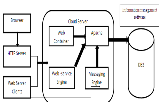
Fig 3. System Architecture
