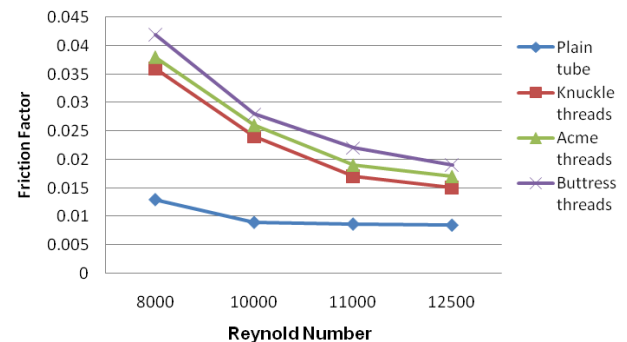
Fig. 6 shows the variation of friction factor Vs Reynolds number for the plain tube and three different test tubes
