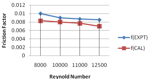
Fig. 4 Validation of numerical results for friction factor of plain pipe against existing correlation
