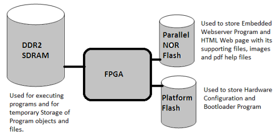
Figure 2 : Memory Interconnection with FPGA
