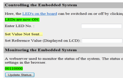
Figure 5 : Magnified view of the web page loaded in Internet Explorer
