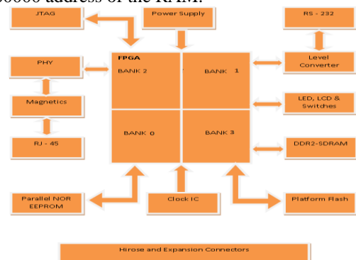
Figure 3 : Block Diagram of Developed Card
