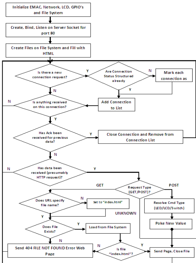
Figure 4 : Webserver Flow Chart
