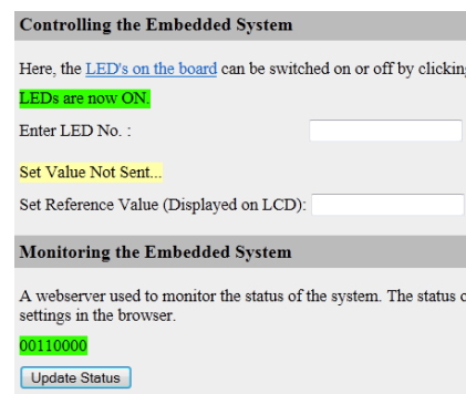
Figure 5 : Magnified view of the web page loaded in Internet Explorer
