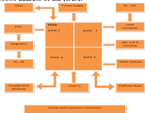
Figure 3 : Block Diagram of Developed Card
