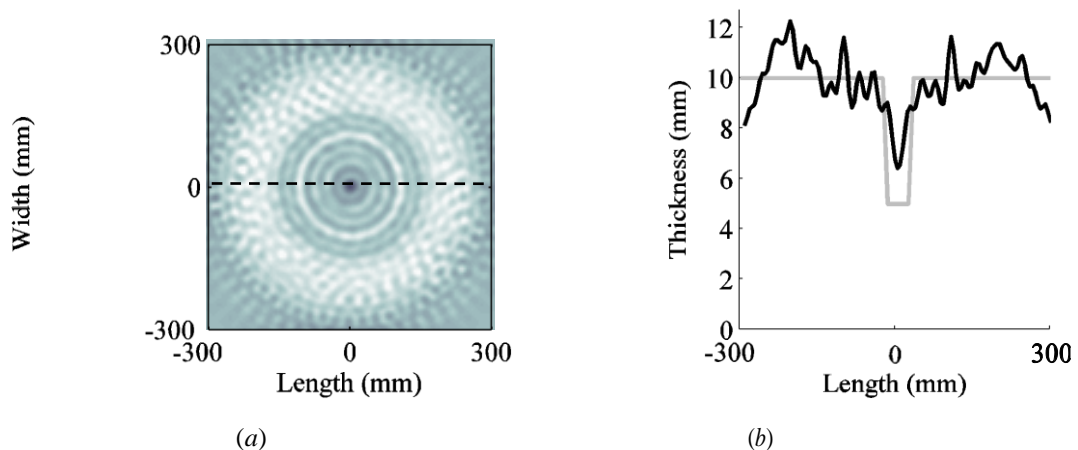
Figure 4: Experimental polychromatic diffraction tomography reconstruction between 45 and 55 kHz with one thickness reduction at the centre of the array and using only the transmission data of the total field (a) Map of the reconstructed thickness and (b) thickness profile across the defect. The black line corresponds to the reconstructed thickness profile and the grey line to the actual thickness profile.
