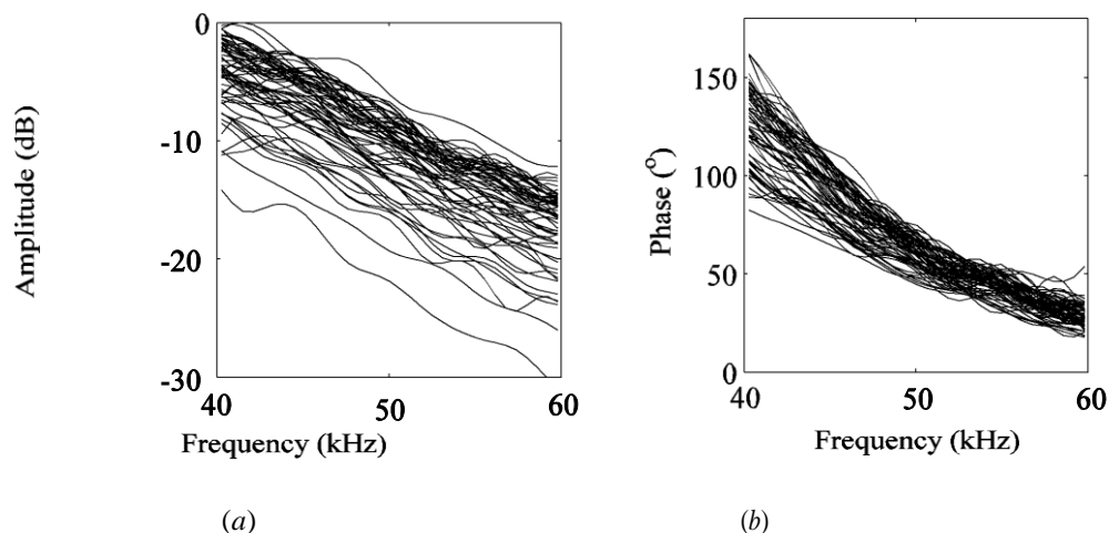
Figure 2: Frequency response functions between the input to the transducer and the displacement measured on top of the transducer for the 64 transducers of the array. (a) Amplitude normalized to maximum in dB and (b) phase in degrees.
