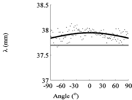
Figure 3: Variation of the wavelength of the A0 mode in the plate as a function of the angle of propagation in degrees. The black line corresponds to a polynomial fit of the wavelength measured (black dots) on the plate and light grey line corresponds to the theoretical value of the wavelength for this type of aluminium..
