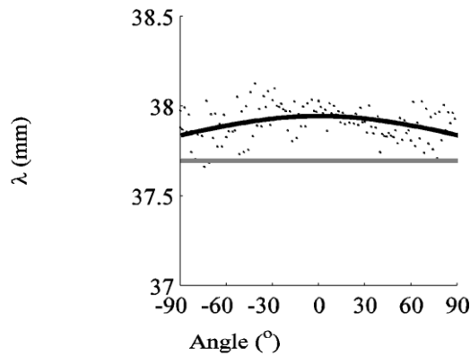
Figure 3: Variation of the wavelength of the A0 mode in the plate as a function of the angle of propagation in degrees. The black line corresponds to a polynomial fit of the wavelength measured (black dots) on the plate and light grey line corresponds to the theoretical value of the wavelength for this type of aluminium..
