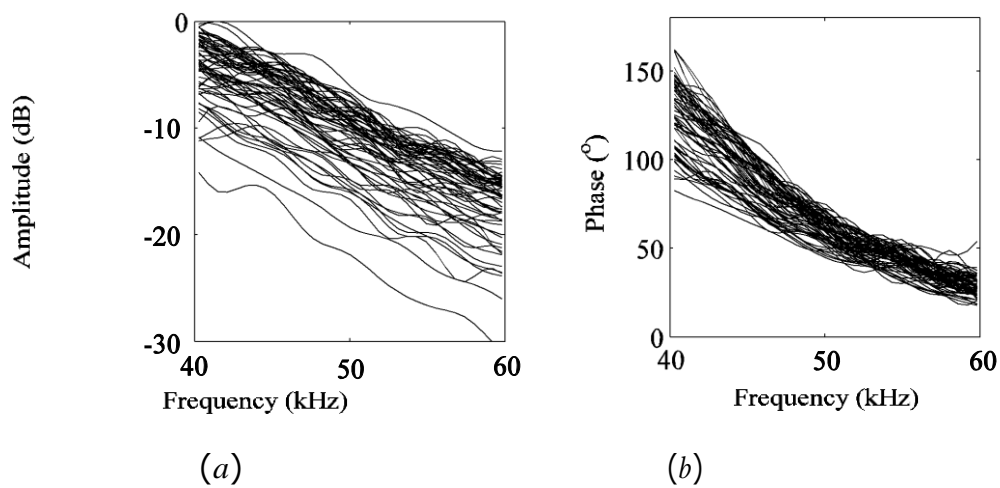
Figure 2: Frequency response functions between the input to the transducer and the displacement measured on top of the transducer for the 64 transducers of the array. (a) Amplitude normalized to maximum in dB and (b) phase in degrees.
