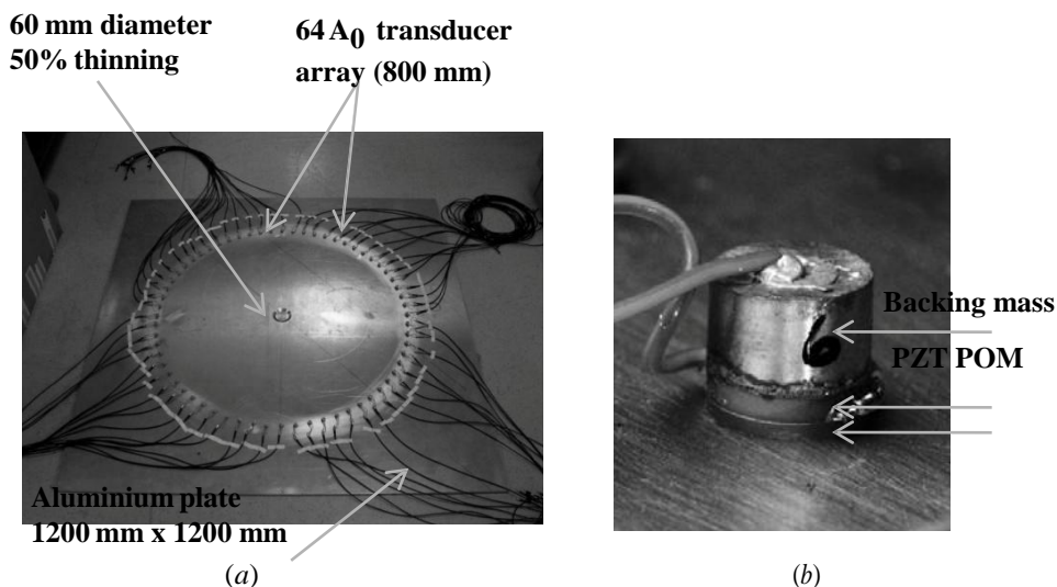
Figure 1: (a) Photograph of the experimental setup with a single defect in the centre of array. (b) Zoom on one of the transducer composed of three layers: a backing mass, a piezoceramic element (PZT) and a layer of polyoxymethylene plastic (POM).
