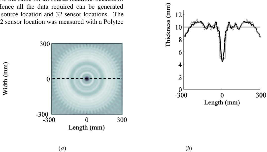
Figure 5: Experimental polychromatic diffraction tomography reconstruction between 45 and 55 kHz with one thickness reduction at the centre of the array and using only the transmission data of the total field (a) Map of the reconstructed thickness and (b) thickness profile across the defect. The measurement is carried out with a Polytec laser vibrometer.
