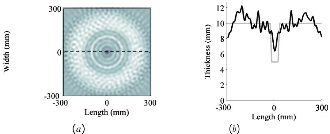
Figure 4: Experimental polychromatic diffraction tomography reconstruction between 45 and 55 kHz with one thickness reduction at the centre of the array and using only the transmission data of the total field (a) Map of the reconstructed thickness and (b) thickness profile across the defect. The black line corresponds to the reconstructed thickness profile and the grey line to the actual thickness profile.
