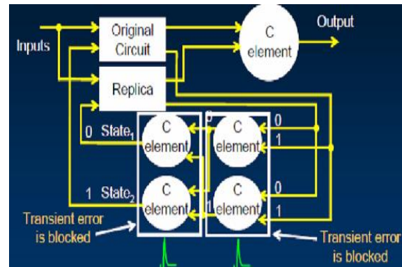
Fig.2:Tolerating Error on state-line C-Element
