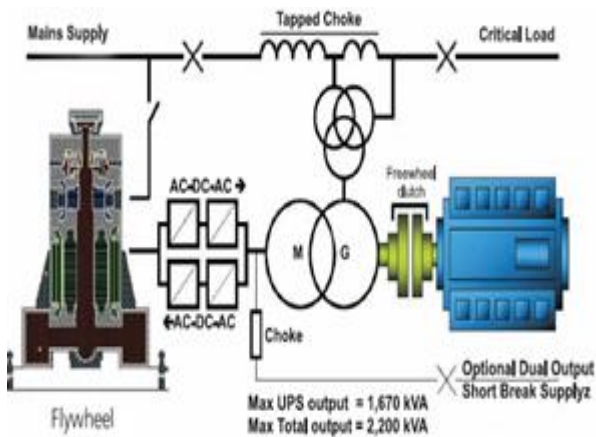
[Fig.-3: Schematic of Rotary UPS System]
