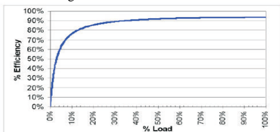
Fig 2: Loading v/s Efficiency graph
