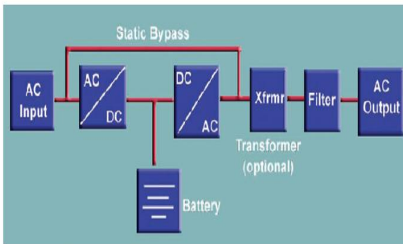
Fig 1: UPS system
