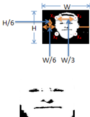
Fig 3.2 Face recognition
