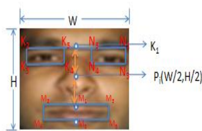
Fig 3.3.1 Feature Extraction
