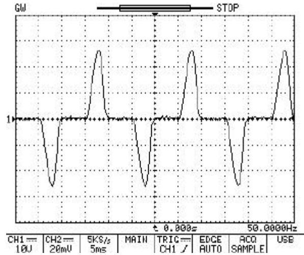
Fig. 12. Experimental waveform of nonlinear load current.
