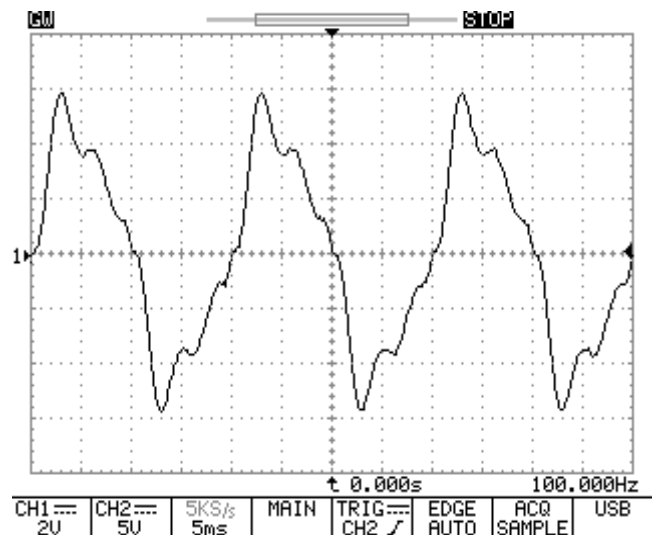
Fig. 13. Experimental waveform of the power source current with the passive filter only.
