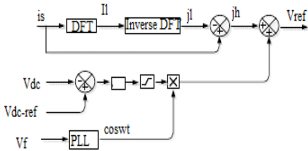
Fig. 2. Control circuit of hybrid series active filter.
