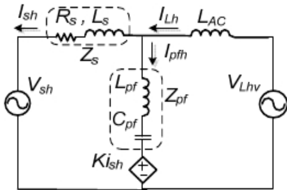
Fig. 7. Harmonic equivalent circuit of single phase system.
