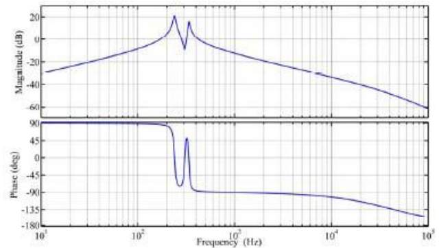
Fig. 6. System frequency response.
