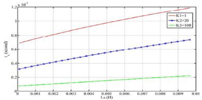
Fig. 5. Relationship between system critical time and system impedance.
