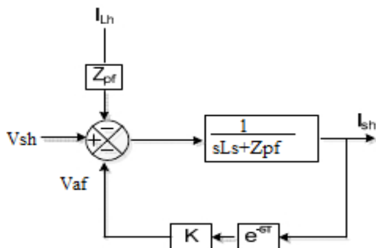
Fig. 4. Control diagram of the system with constant delay
