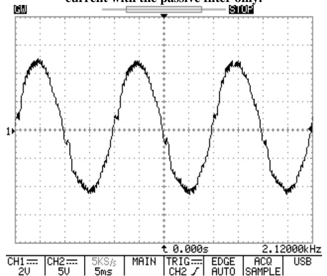
Fig. 14. Experimental waveform of the power source current with both the active and the passive filter.
