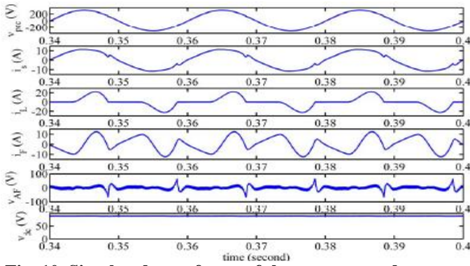
Fig. 10. Simulated waveforms of the compensated system with the hybrid series active filter.
