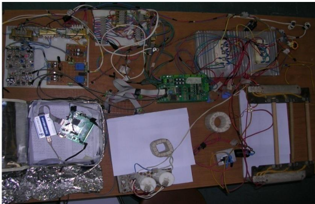
Fig. 11. Laboratory 220 V – 2.2 kW hybrid series active filter.
