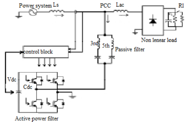
Fig. 1. System configuration
