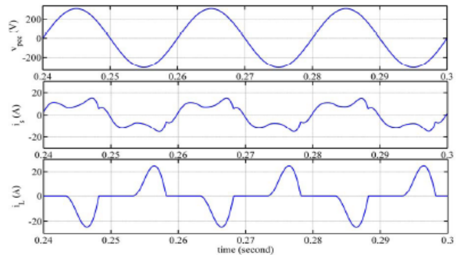
Fig. 9. Simulated waveforms of compensated system with passive filter.
