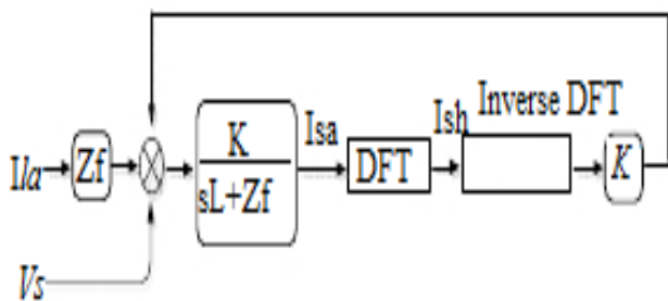
Fig. 3. Block diagram of the whole system.
