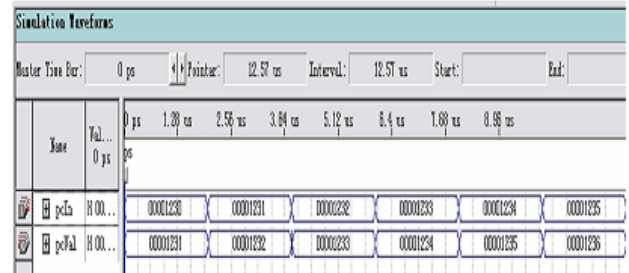
Figure. 16 incPC Module Simulation Waveform
