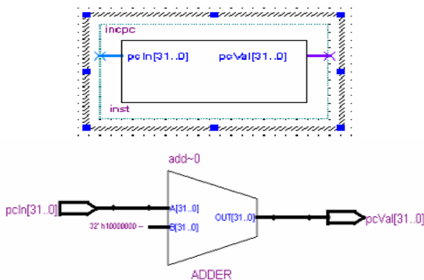
Figure. 15 incPC Entity Structure and RTL Structure
