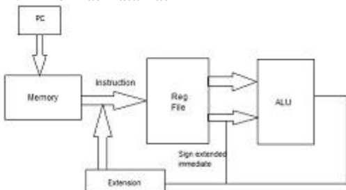
Figure. 3 RI-Format Instruction Data Path
