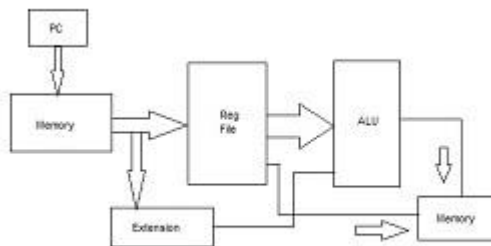
Figure. 5 Memory Instruction Data Path
