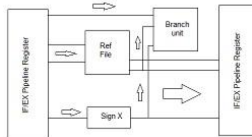
Figure. 8 ID Stage
