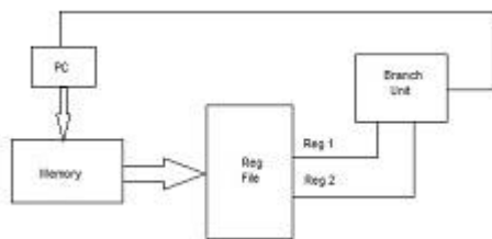
Figure. 6 Jump Instruction Data Path
