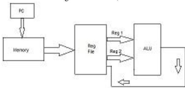
Figure. 2 R-Format Instruction Data Path
