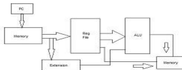
Figure. 4 Load Word Data Path
