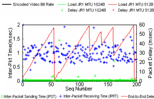
Fig. 3(a) Per-Packet Delay and Inter-Packet Time (b) Close-up view of the first video frame
