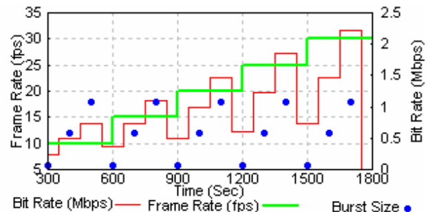
Fig. 5: Offered CBR traffic
