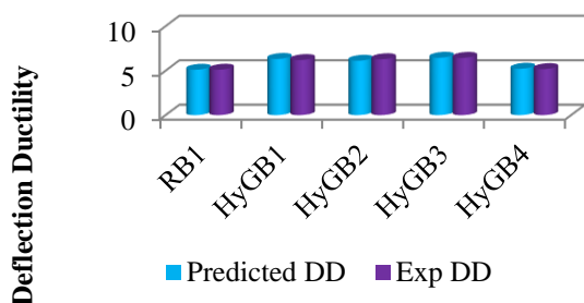
Fig. 10 Experimental vs Predicted results for Deflection Ductility
