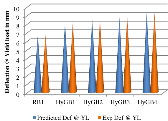
Fig. 5 Experimental vs Predicted results for Deflection at Yield Load
