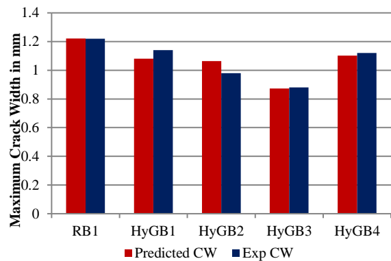
Fig. 12 Experimental vs Predicted results for Maximum Crack Width
