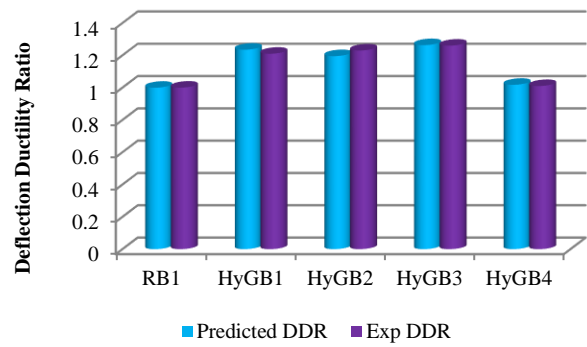
Fig. 11 Experimental vs Predicted results for Deflection Ductility Ratio
