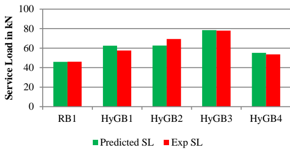
Fig. 6 Experimental vs Predicted results for Service Load
