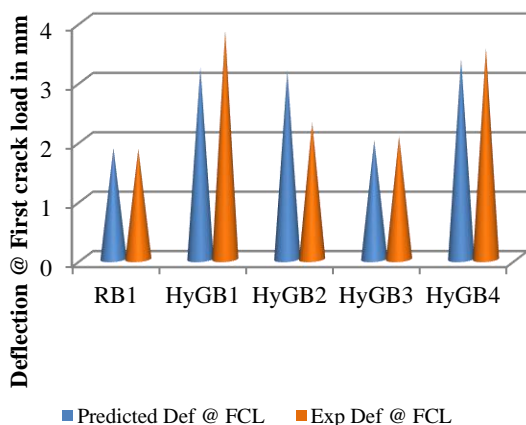
Fig. 3 Experimental vs Predicted results for Deflection at First Crack Load
