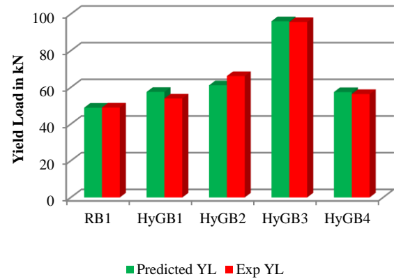
Fig. 4 Experimental vs Predicted results for Yield Load
