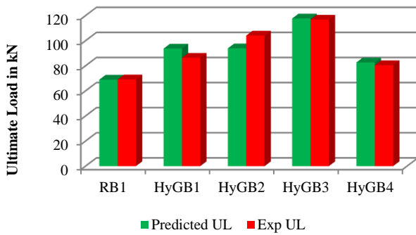
Fig. 8 Experimental vs Predicted results for Ultimate Load
