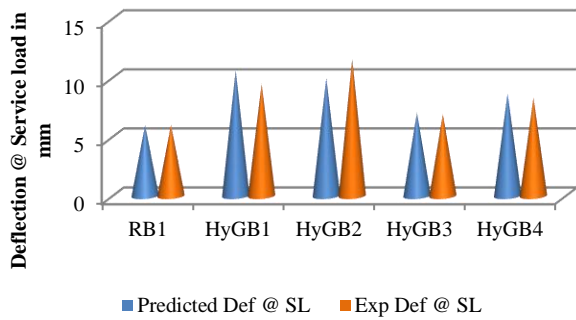
Fig. 7 Experimental vs Predicted results for Deflection at Service Load
