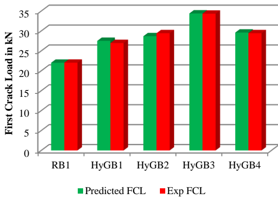
Fig. 2 Experimental vs Predicted results for First Crack Load
