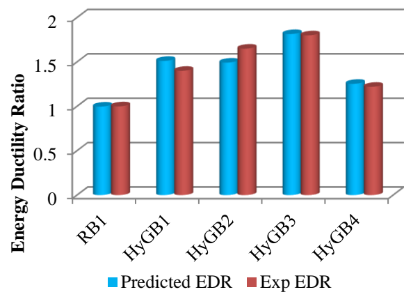
Fig. 13 Experimental vs Predicted results for Energy Ductility Ratio
