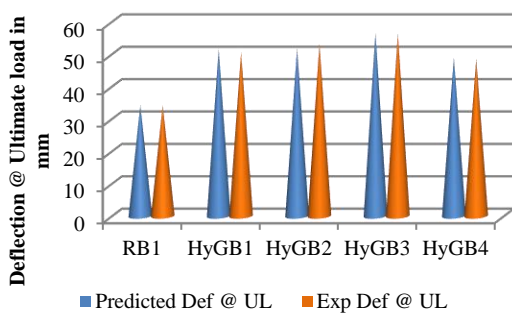
Fig. 9 Experimental vs Predicted results for Deflection at Ultimate Load
